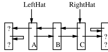
Figure 5. A deque containing three elements.
