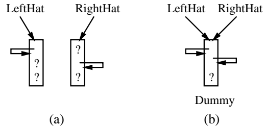
Figure 6. Empty deque states. (a) Generic empty state. (b) Special case empty state.
