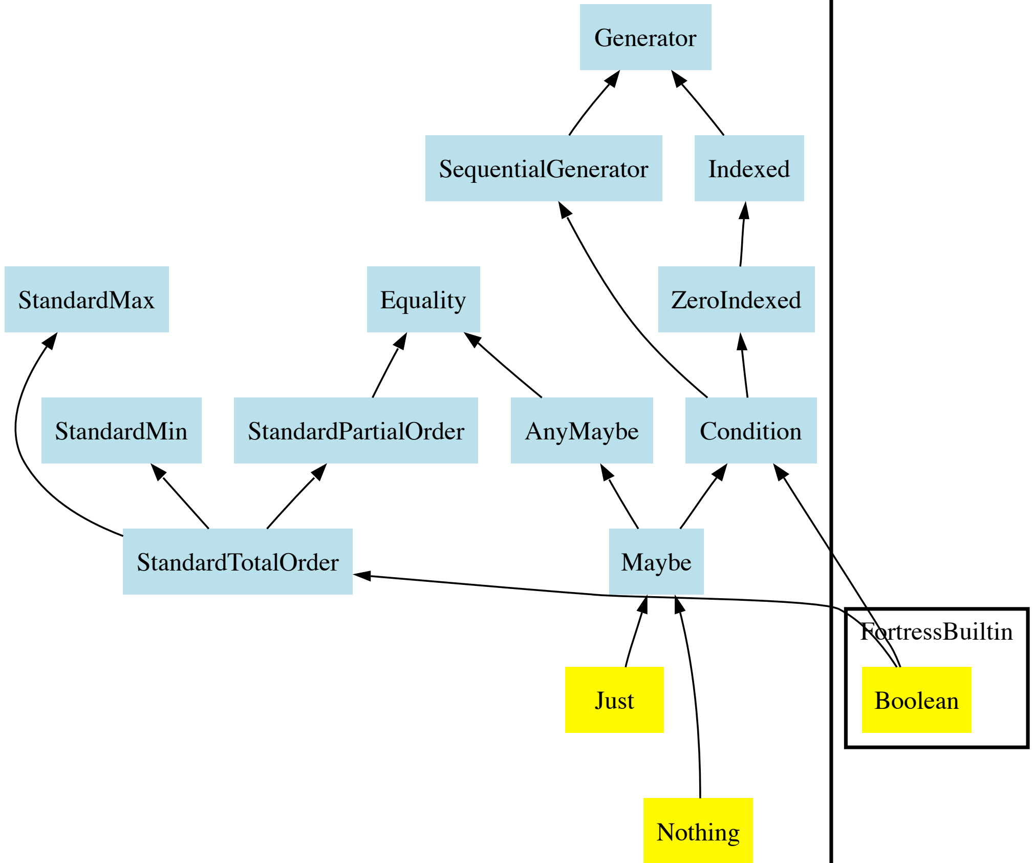
Class dependencies
