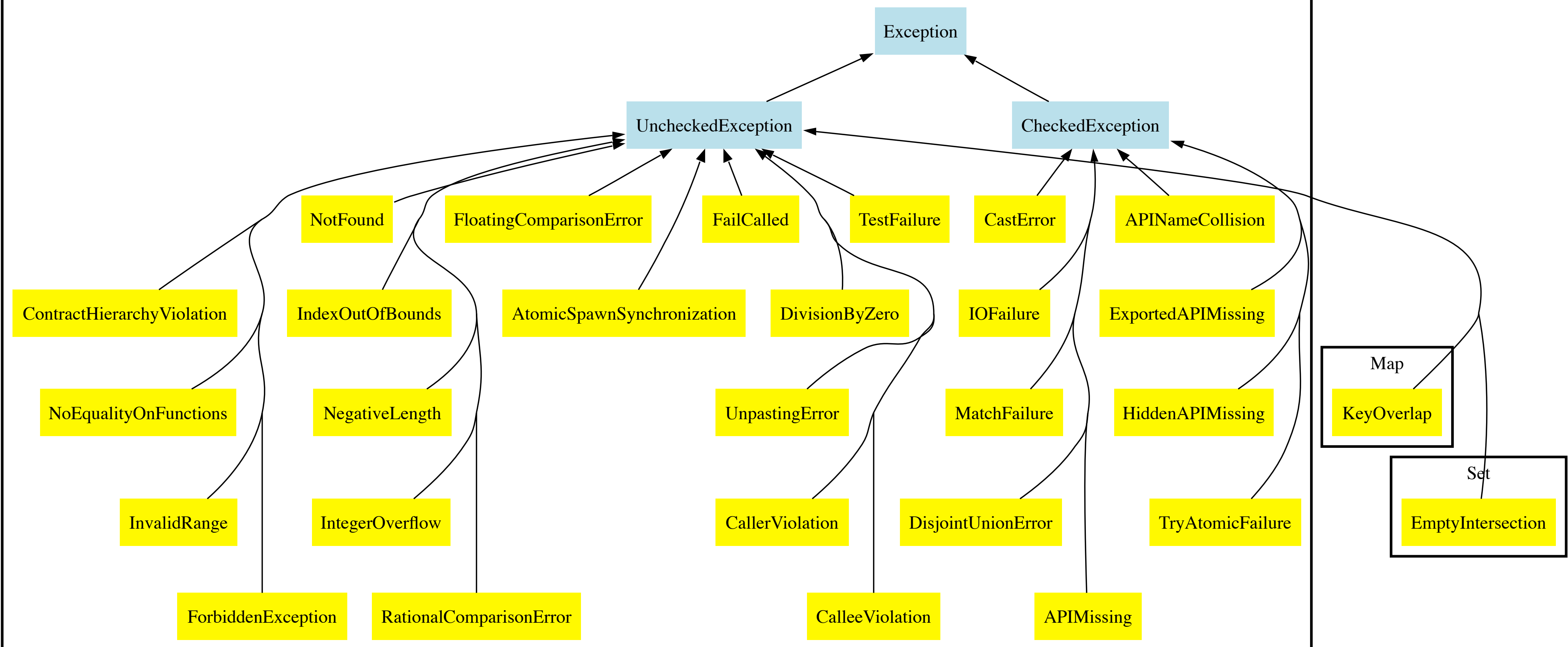
Class dependencies
