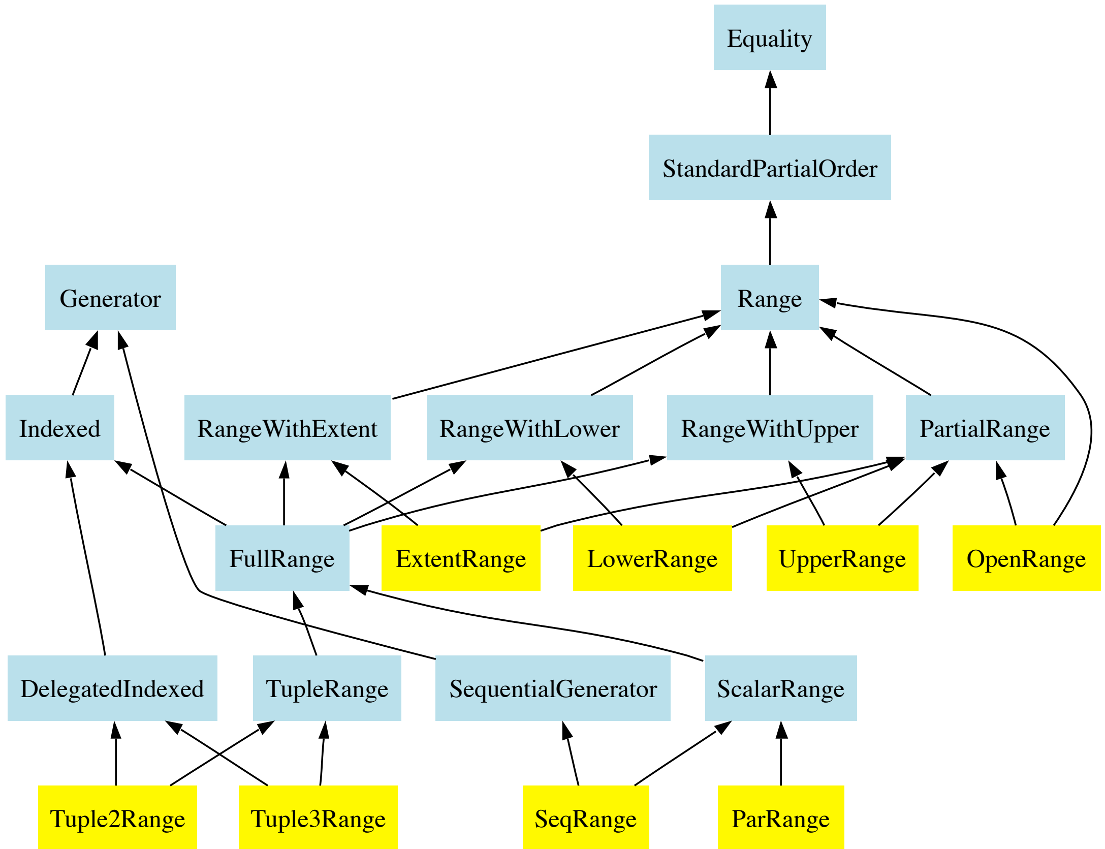
Class dependencies
