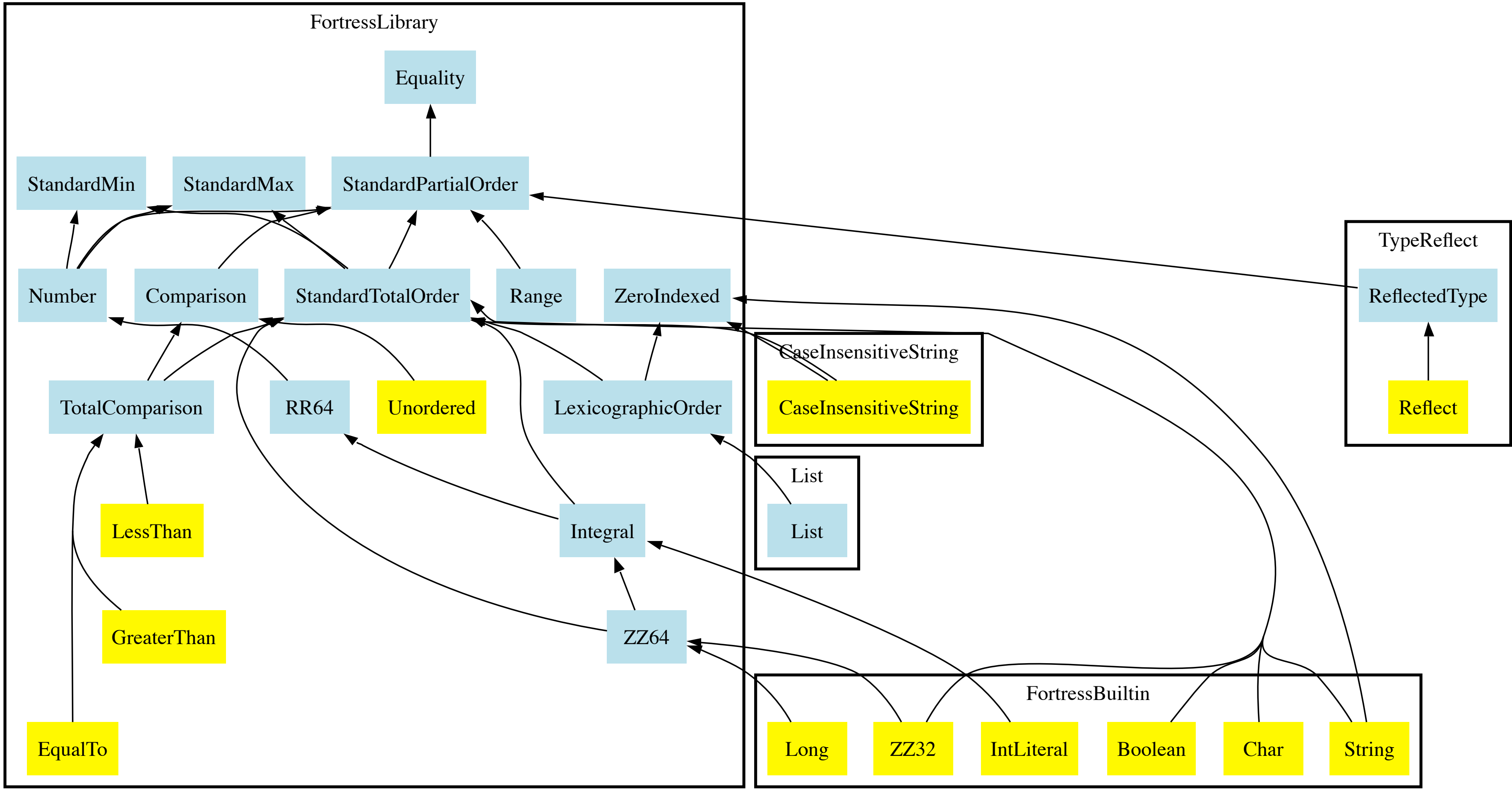
Class dependencies
